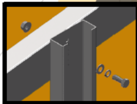
Post connections to Rafter
