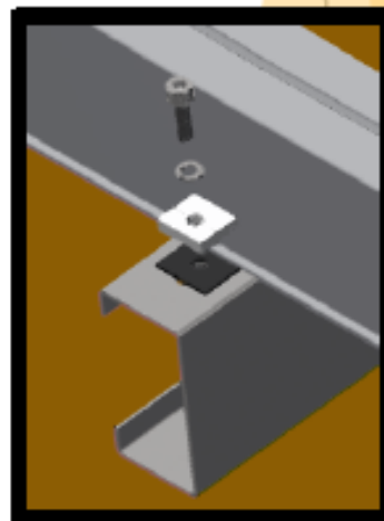
Rail connections to Rafter
